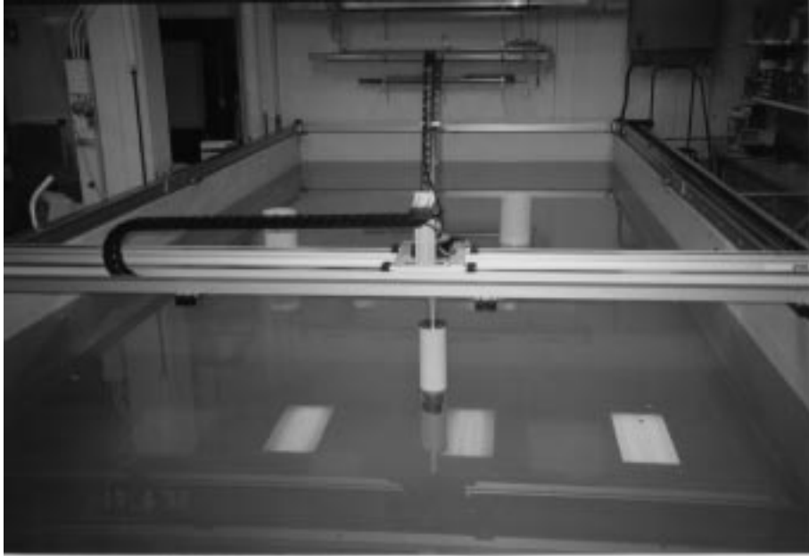
Figure 12: The planar robotic positioning system and sector-scan sonar used in the underwater sonar experiments. The water in the tank is approximately 1 meter deep. The transducer was translated and rotated in a horizontal plane mid-way through the water column.
